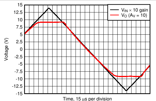
V_{IN} = 2.8\text{-V}_{PP} triangular waveform
