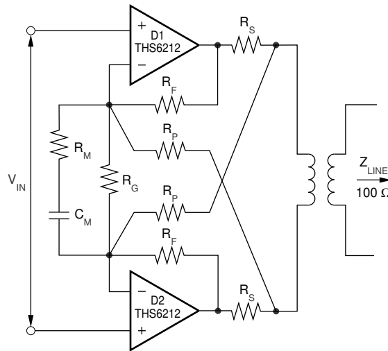
Figure 8-7. 0.1-dB Flatness Compensation Circuit
