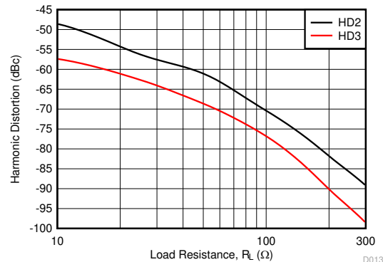
f = 10 MHz, V_O = 2\text{ V}_{PP} , A_V = 10\text{ V/V}
