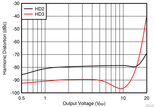
f = 1 MHz, A_V = 10\text{ V/V}
