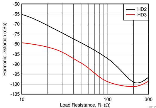
f = 1 MHz, V_O = 2\text{ V}_{PP} , A_V = 10\text{ V/V}
